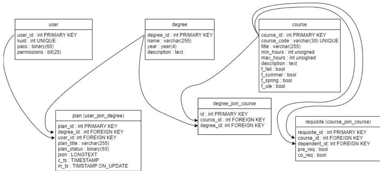
Figure 2 : Database Table Structure
